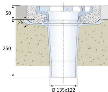
Base assembly with one riser
