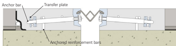
WRB with anchor bars
